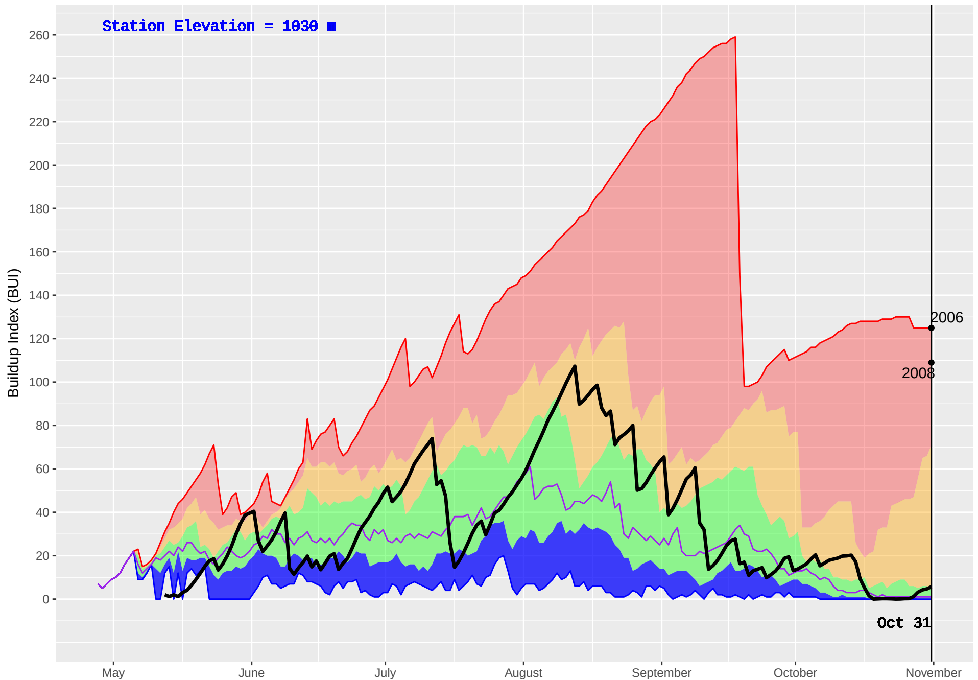
WITCH (154) : Historical (1993–2016) and Current (2017) Noon Buildup Index (BUI)
