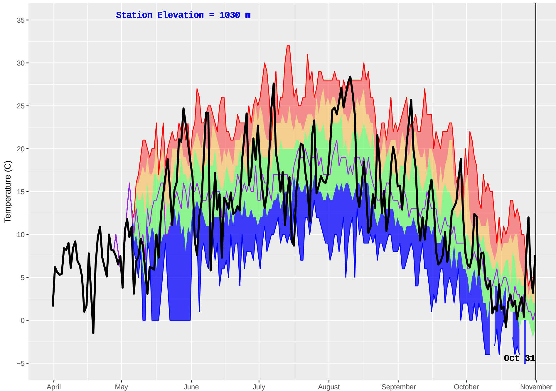
WITCH (154) : Historical (1993–2016) and Current (2017) Noon Temperature
