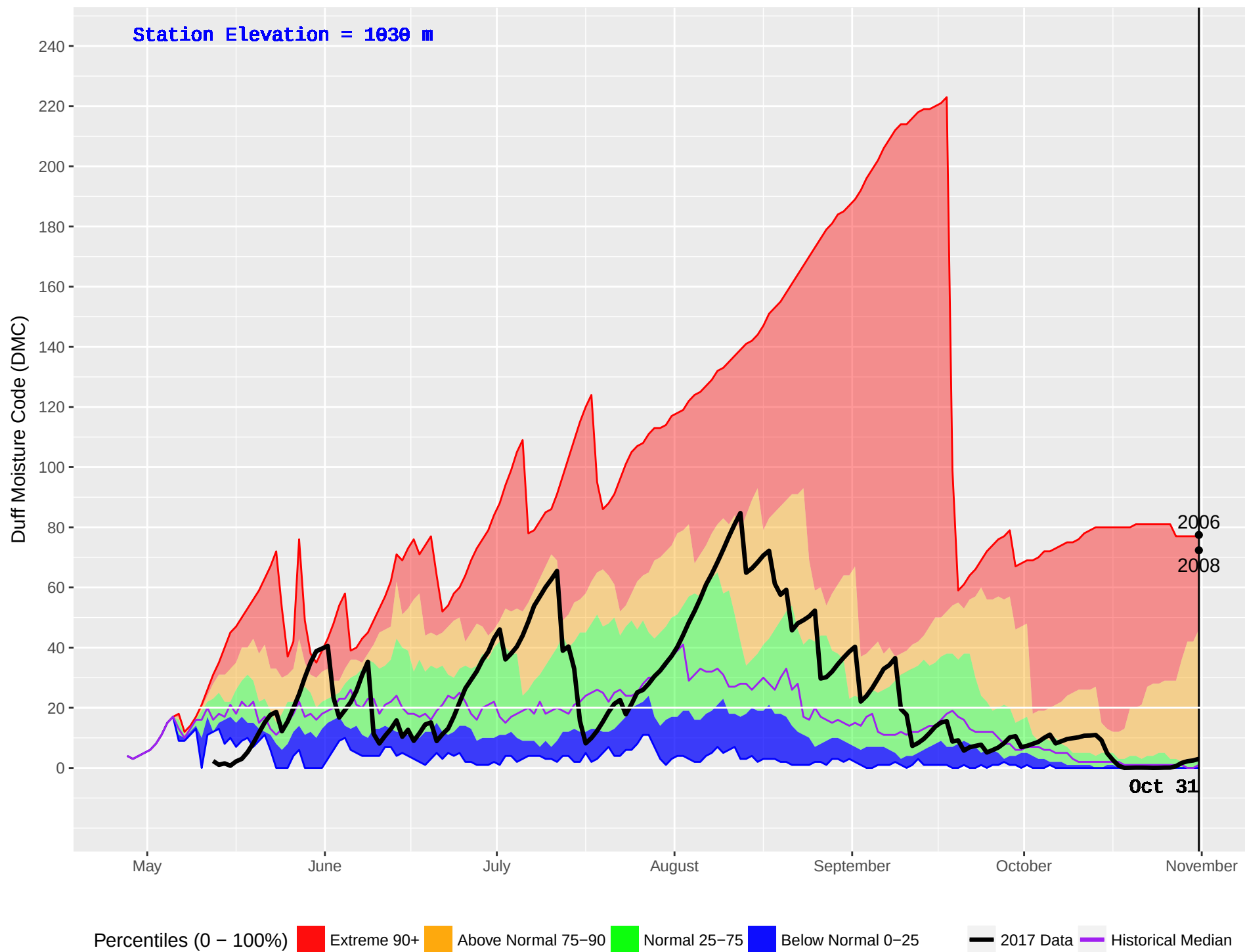
WITCH (154) : Historical (1993–2016) and Current (2017) Noon Duff Moisture Code (DMC)
