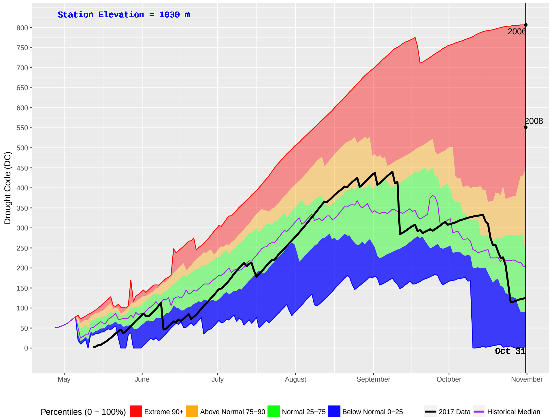
WITCH (154) : Historical (1993–2016) and Current (2017) Noon Drought Code (DC)
