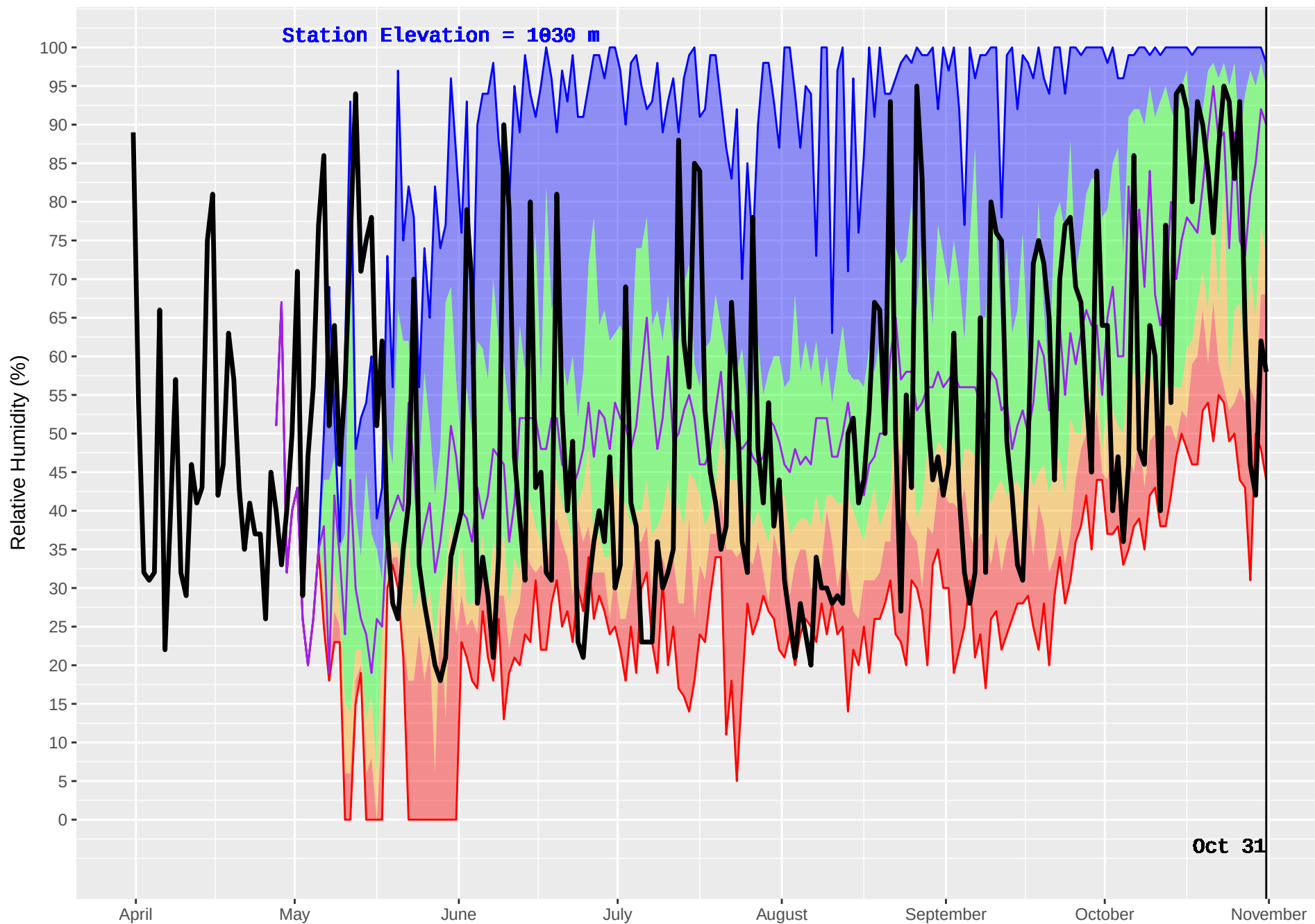
WITCH (154) : Historical (1993–2016) and Current (2017) Noon Relative Humidity
